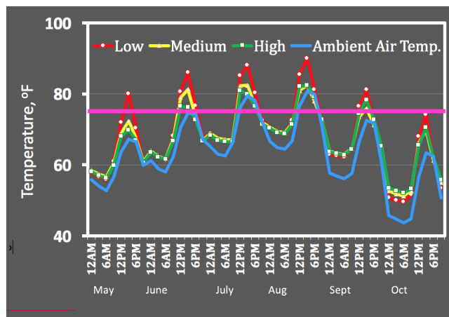
Figure 6. This graph shows average air temperature (blue line) and the average soil temperatures under low (red), moderate (yellow), and high (green) shade conditions in young stands of walnut and honeylocust trees. Temperatures were averaged over 24 hours within months in 2003, a relatively cool year. The pink line at about 75 degrees Fahrenheit (°F) represents the optimal temperature for cool-season grass growth (Sprague 1944). Graph reprinted by permission from Buerger (2004).
